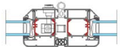
Interlock Detail
